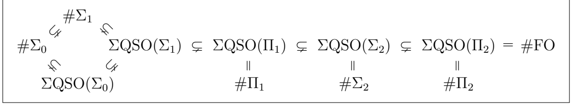
FIGURE 5.1. The relationship between the #FO-hierarchy and the \Sigma \text{QSO}(\text{FO}) -hierarchy, where \# \Sigma_1 and \Sigma \text{QSO}(\Sigma_0) are incomparable.
